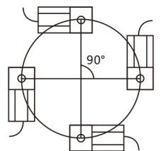
切向安装 Tangential mounting
